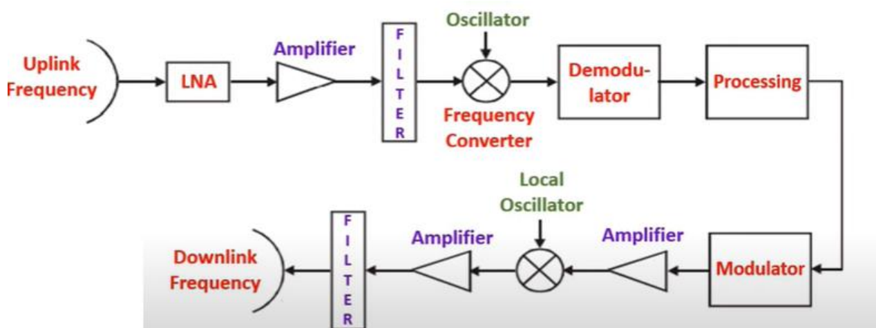
Figure 4 – Satellite Transponder and Reception/Transmission of data, [SatNow]
